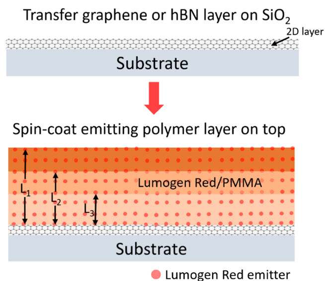
Figure 3. Schematic of the 2D layer/emitting polymer sample used to extract the fluorescence quenching radius of graphene and h-BN. Lumigen Red/PMMA emitting layers with different thicknesses ( L ) were spin-coated onto the 2D layers, and the average fluorescence lifetime depends on L and the quenching radius ( R_0 ).
